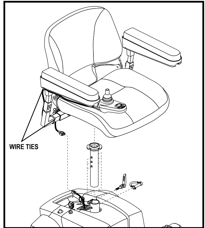
Figure 9. Seat Installation
