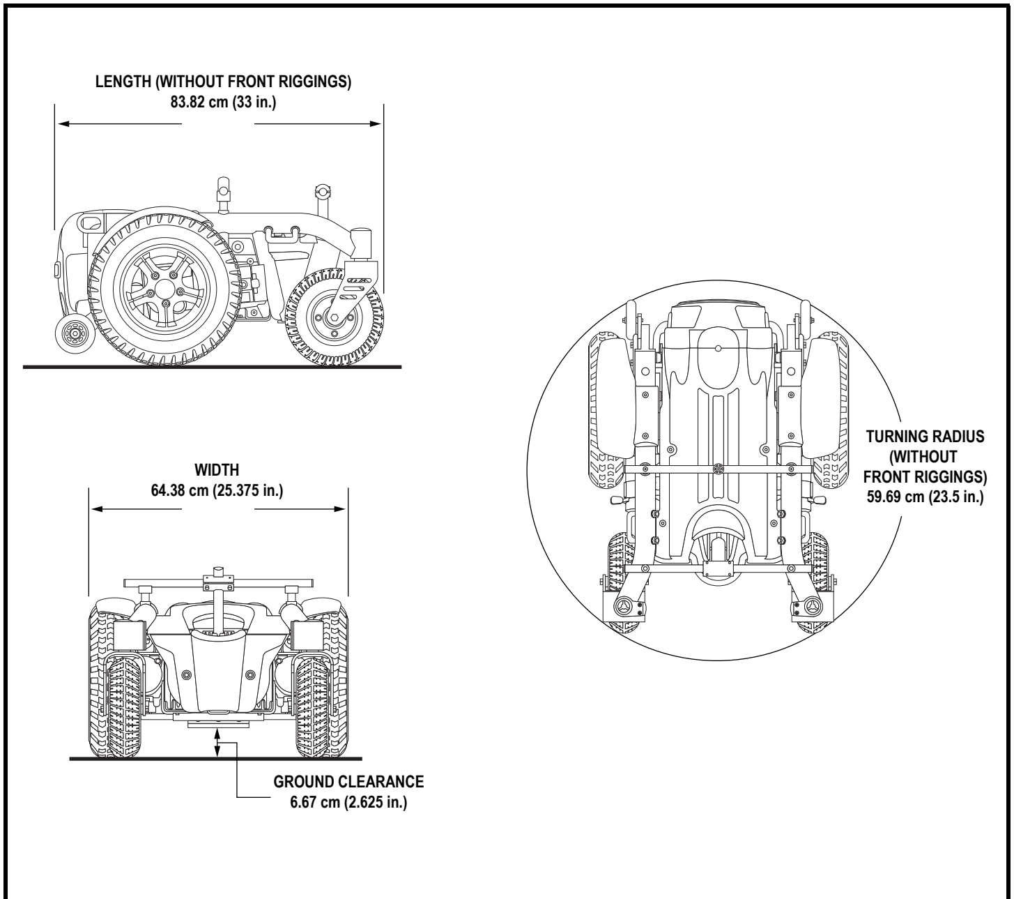
Figure 19. Athena Dimensions and Ground Clearance
