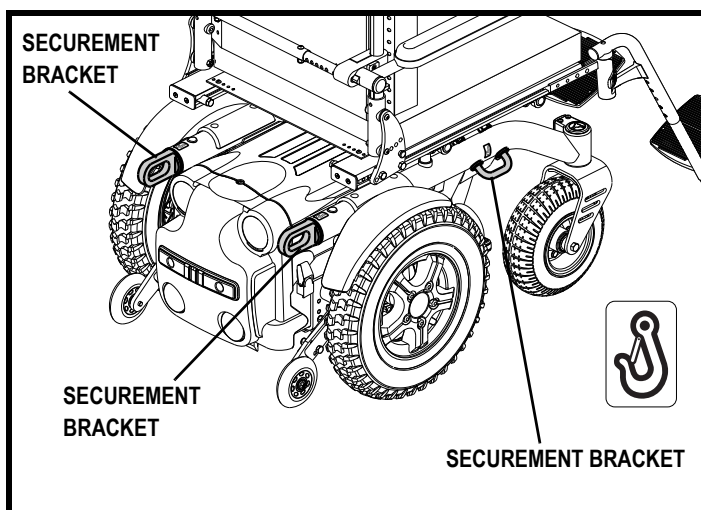
Figure 11. Transit Securement Brackets
